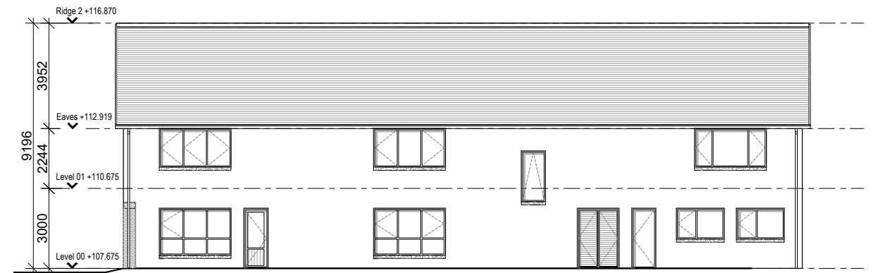
4 West Elevation 0476
