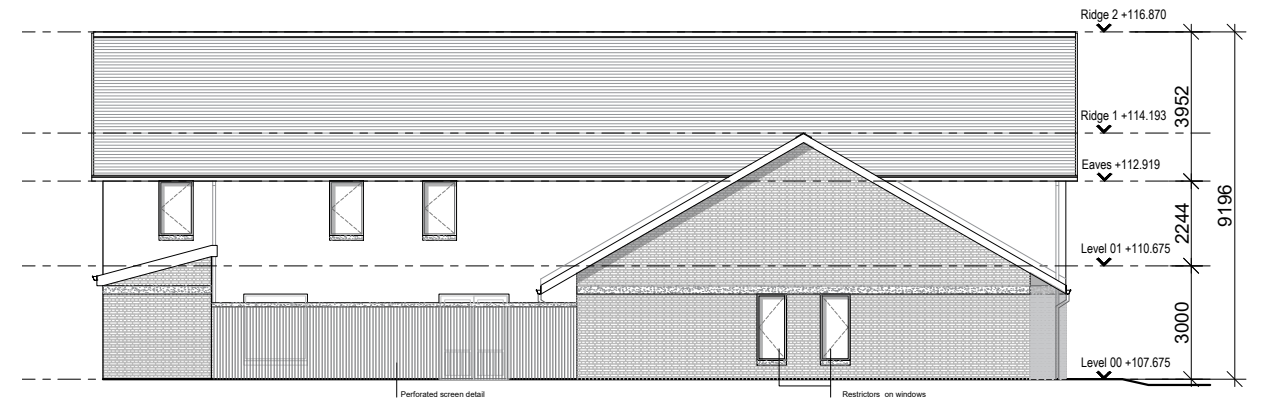
2 East Elevation 0476
