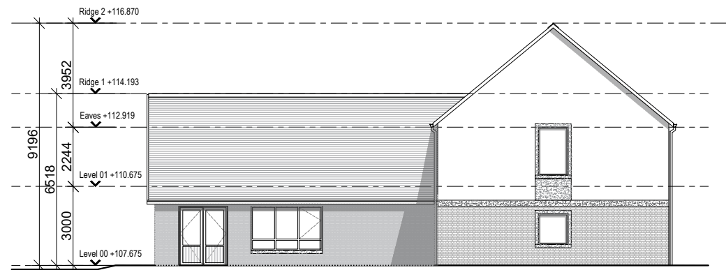
3 North Elevation 0476
